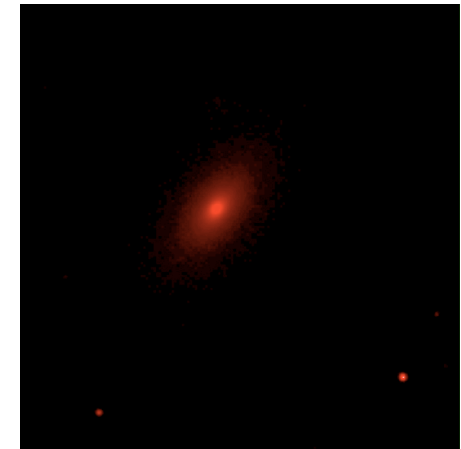
Near-Infrared
