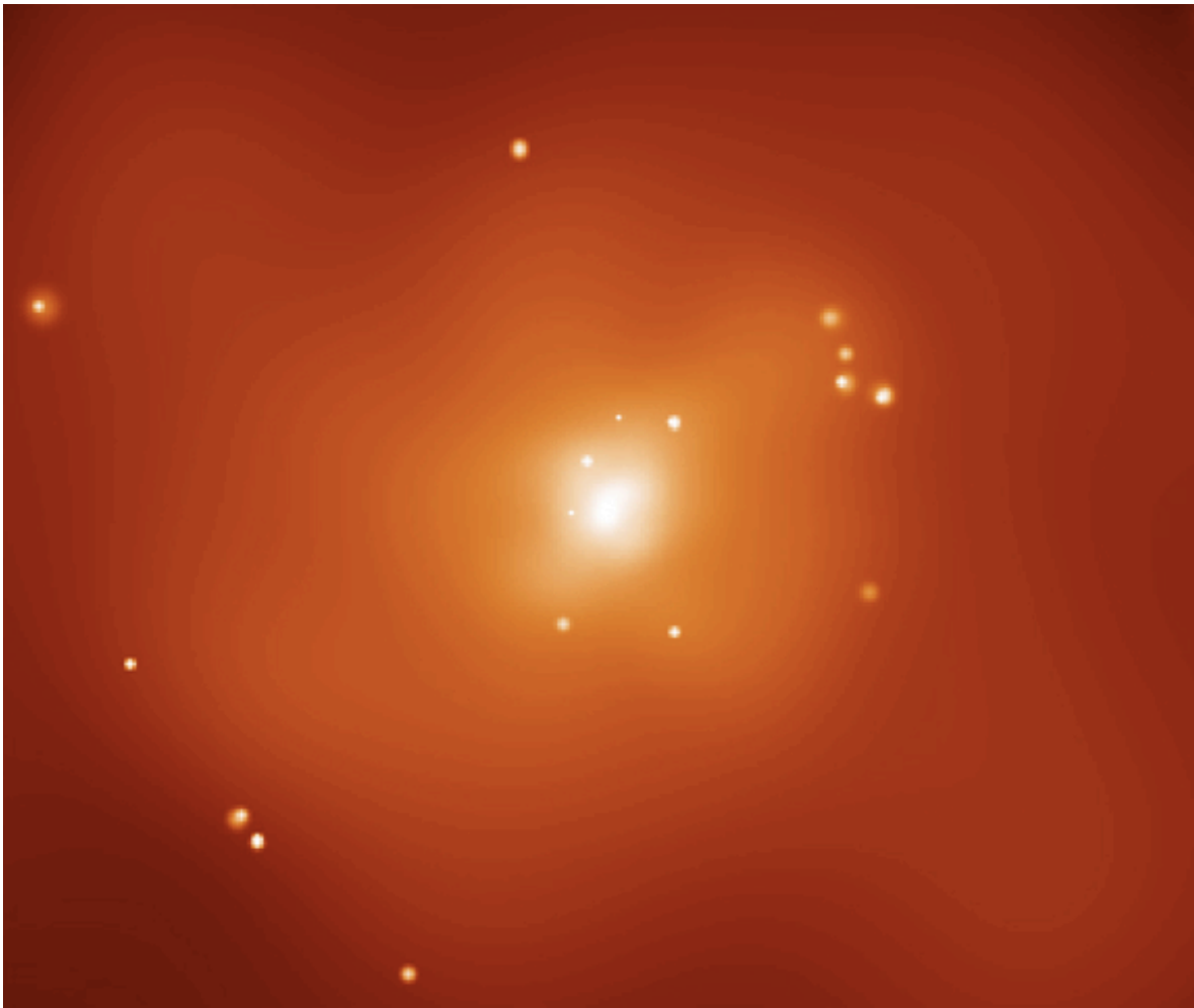
X-ray (Chandra)
