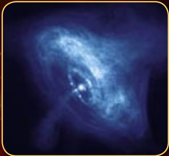
Crab Nebula
