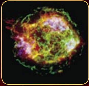
Cassiopeia A
